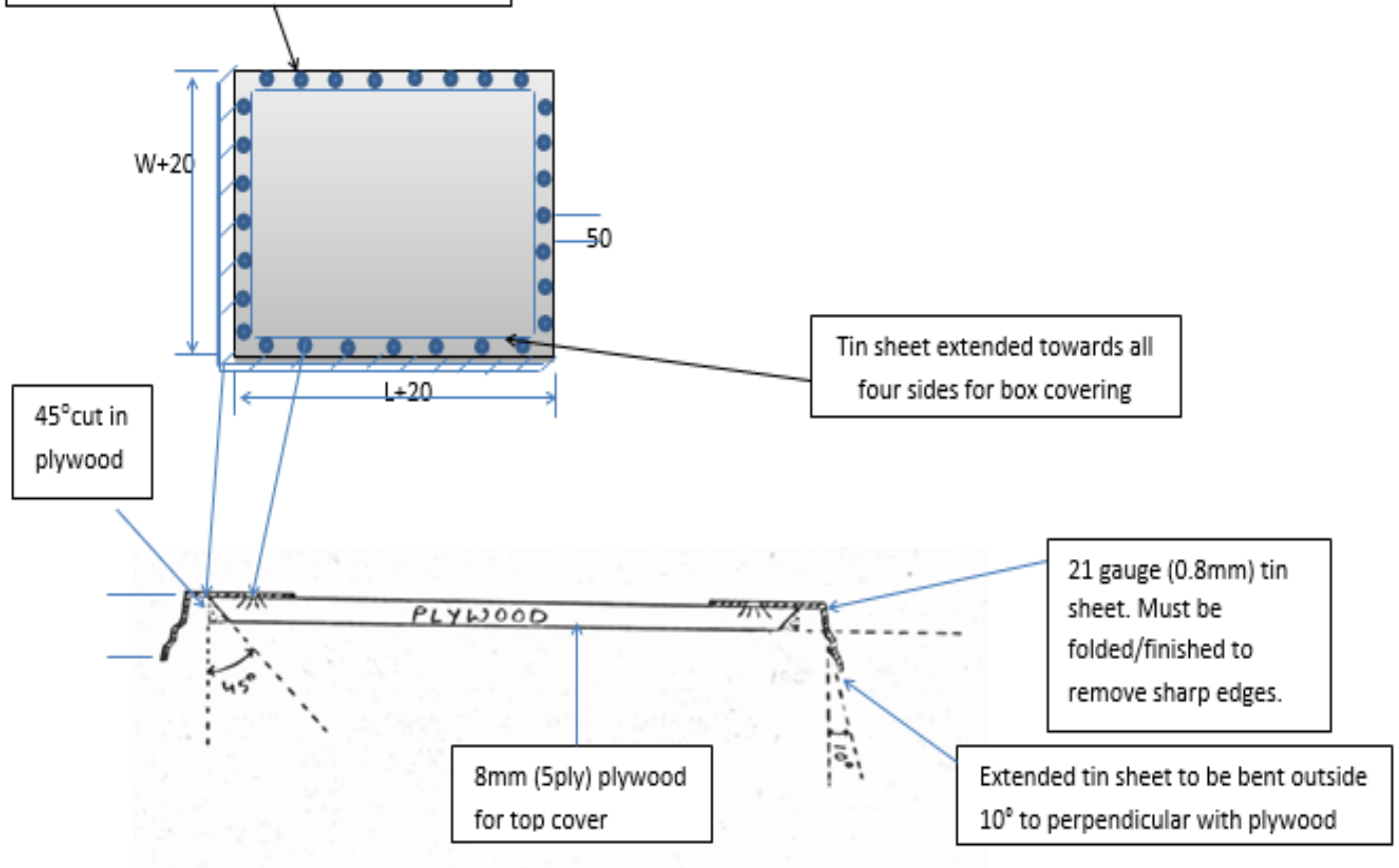
Indicative view for tin sheet fixing
